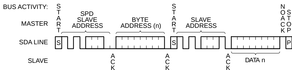
Figure 11a. EEPROM Selective Read
