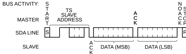
Figure 10b. Temperature Sensor Immediate Read
