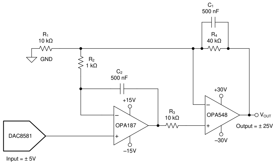
Figure 45. Programmable Power Supply
