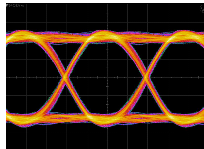
Eye Diagram
