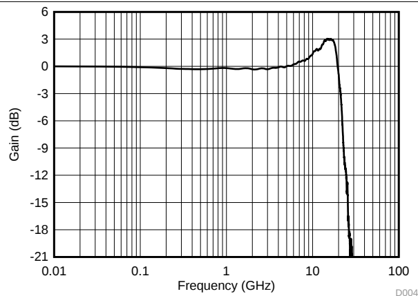
Figure 3. Gain vs Frequency (Test Fixture loss De-embedded)
