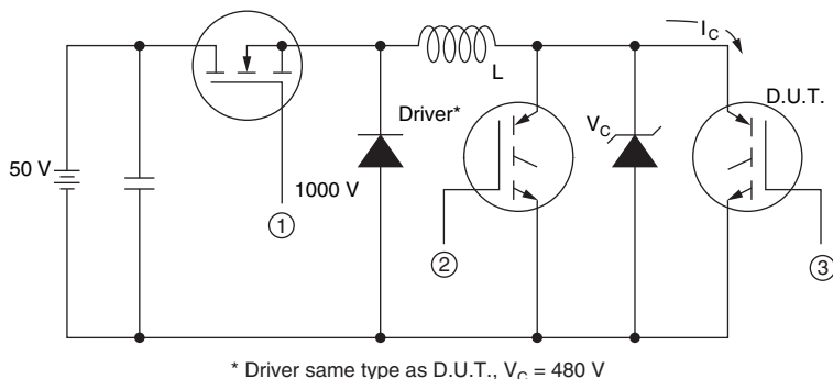
Fig. 18 - Switching Lost Test Circuit
