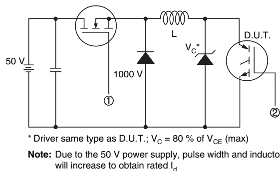
Fig. 16 - Clamped Inductive Load Test Circuit
