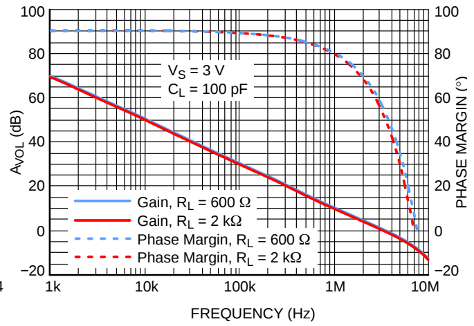
Figure 2. Open Loop Gain and Phase Margin vs. Frequency
