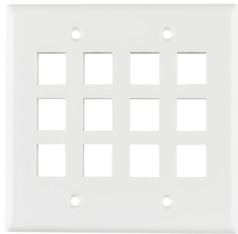
Dual Gang 12 Port Flush Mount Faceplate, ABS 94V-0, White, 1/pkg
