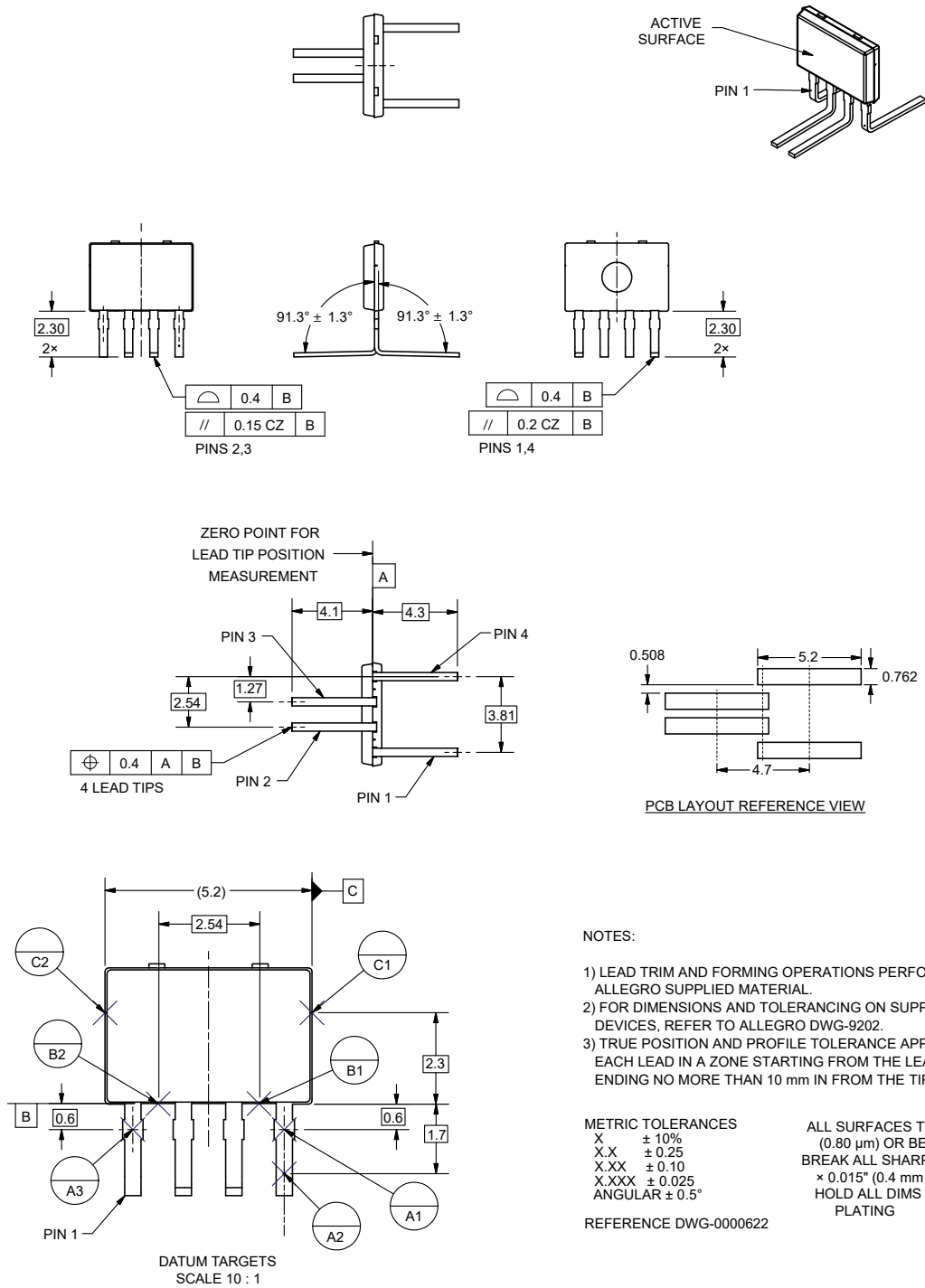
Figure 29: Package KT, 4-Pin SIP, TG Leadform
