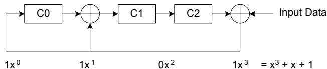
Figure 20: CRC Calculation
