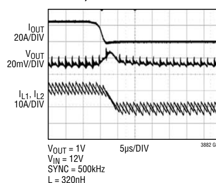
Load Dump Transient Current Sharing (Using FDMF6707B DrMOS)
