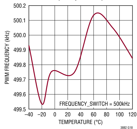
PWM Frequency vs Temperature
