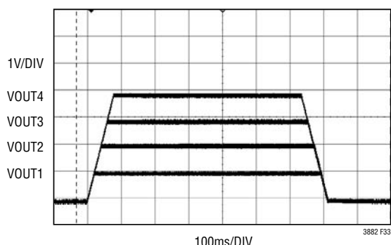
Figure 33. LTC3882 Time-Based Coincident Supply Ramping
