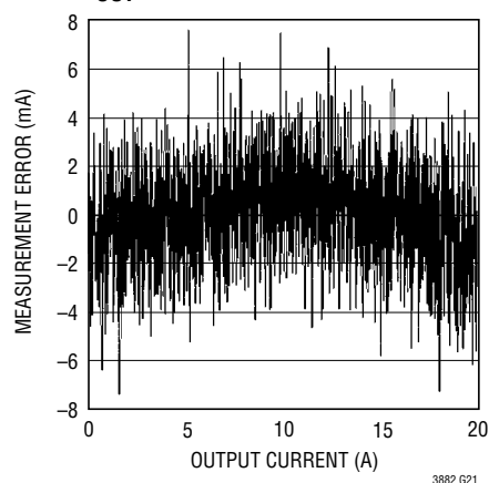
I_{OUT} ADC TUE
