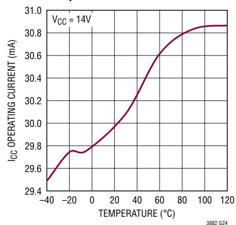
IC Operating Current vs Temperature
