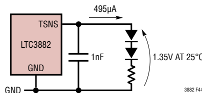
Figure 44. 2D+R Temperature Sense
