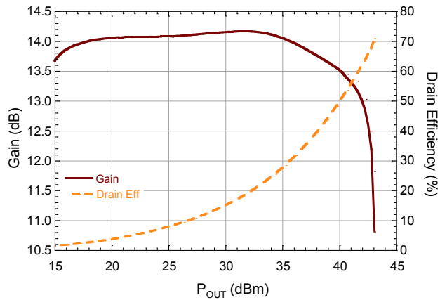
Performance vs. Output Power ( f = 900 MHz)
