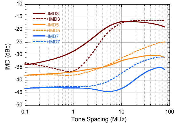
2-Tone IMD vs. Tone Spacing
