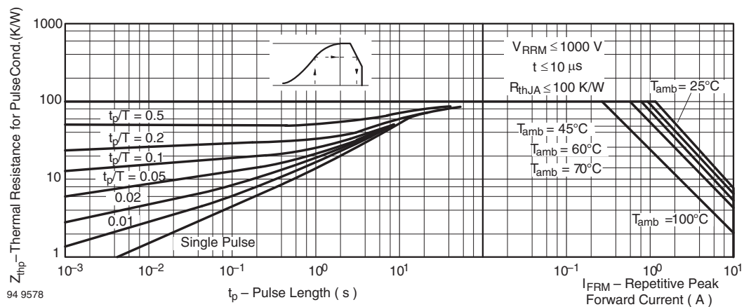
Fig. 6 - Thermal Response
