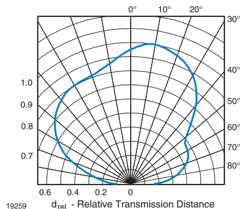
Fig. 13 - Vertical Directivity
