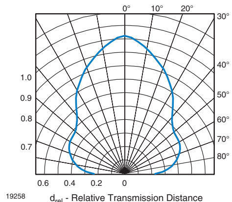
Fig. 12 - Horizontal Directivity
