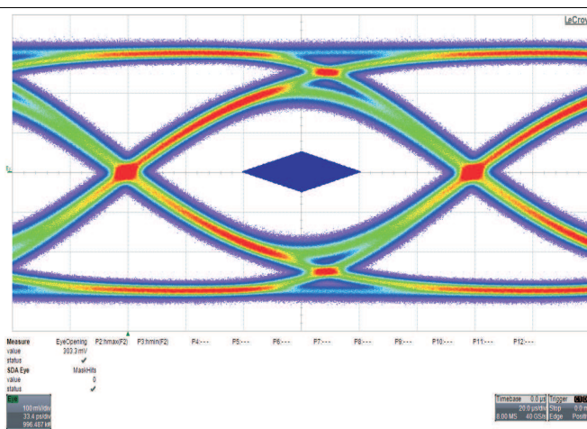
Figure 17. DE = 0 dB, EQ = 7 dB, Input = 12 inches, Output = 8 inches + 3-m Cable
