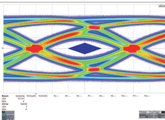
Figure 19. DE = 0 dB, EQ = 7 dB, Input = 12 inches, Output = 16 inches + 3-m Cable
