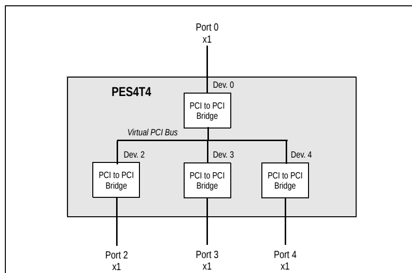
Figure 1.3 PES4T4 Port Configuration
