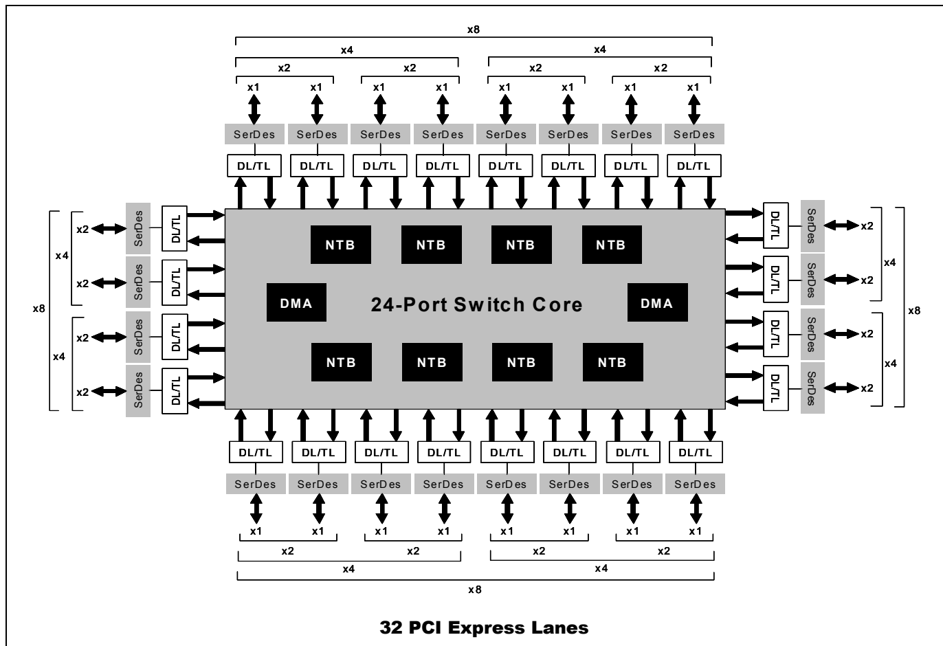
Figure 1 PES32NT24AG2 Block Diagram
