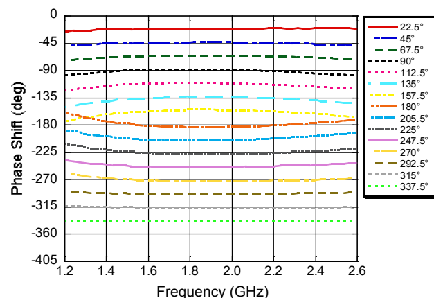
Phase Shift vs. Frequency (All States)
