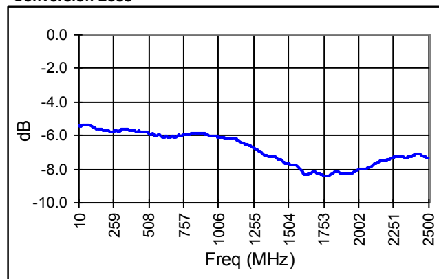
Conversion Loss
