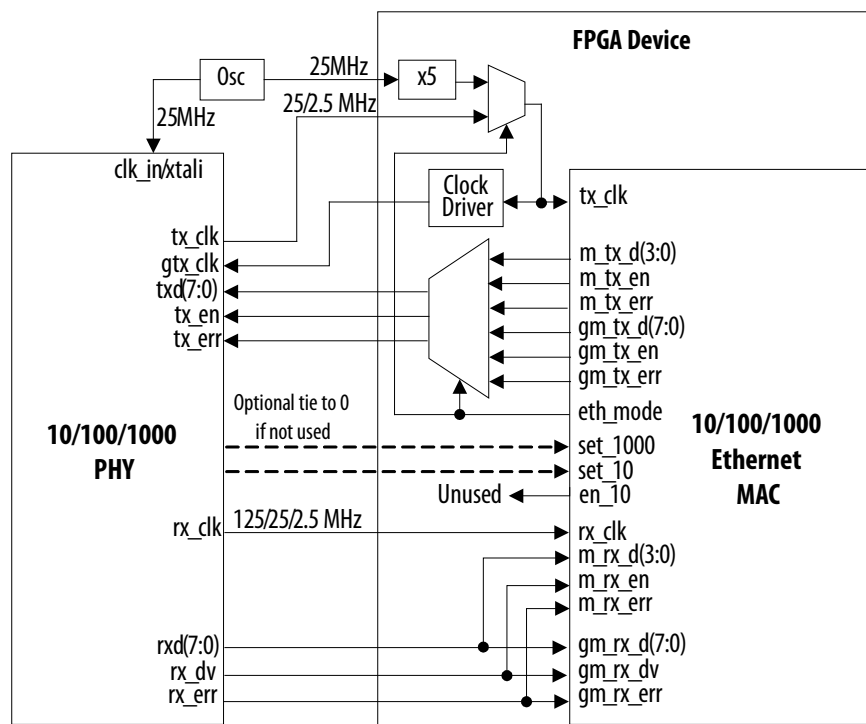
Figure 23. 10/100/1000 PHY Interface via MII/GMII
