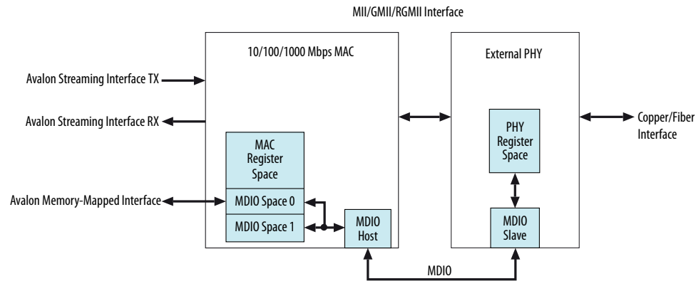
Figure 44. Triple-Speed Ethernet System with MII/GMII or RGMII with Register Initialization Recommendation
