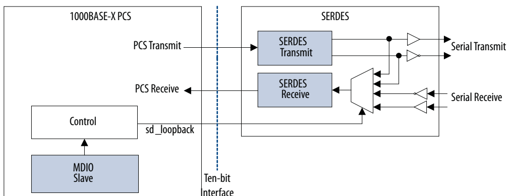
Figure 34. Serial Loopback
