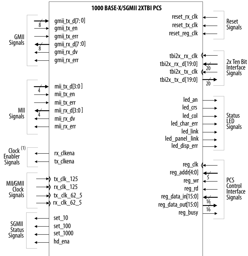
Figure 58. 1000BASE-X/SGMII 2XTBI PCS Function Signals
