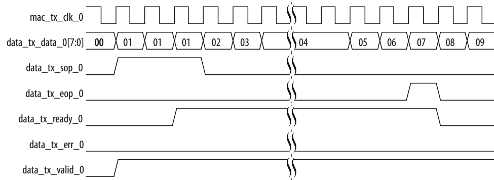
Figure 65. Transmit Operation—MAC Without Internal FIFO Buffers
