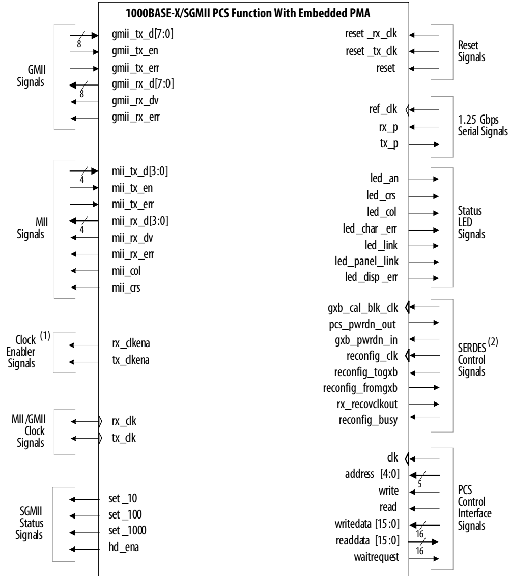
Figure 59. 1000BASE-X/SGMII PCS Function and PMA Signals
