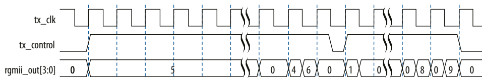
Figure 68. RGMII Transmit with Error in 1000 Mbps
