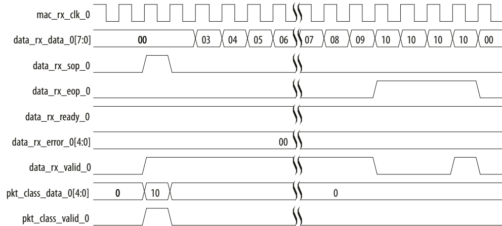
Figure 62. Invalid Length Error During Receive Operation—MAC With Internal FIFO Buffer
