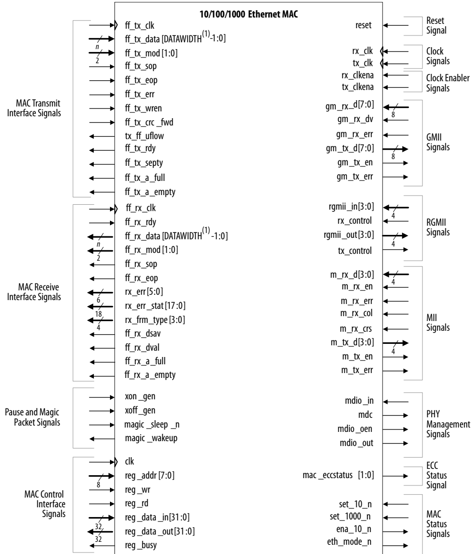
Figure 47. 10/100/1000 Ethernet MAC Function with Internal FIFO Buffers Signals
