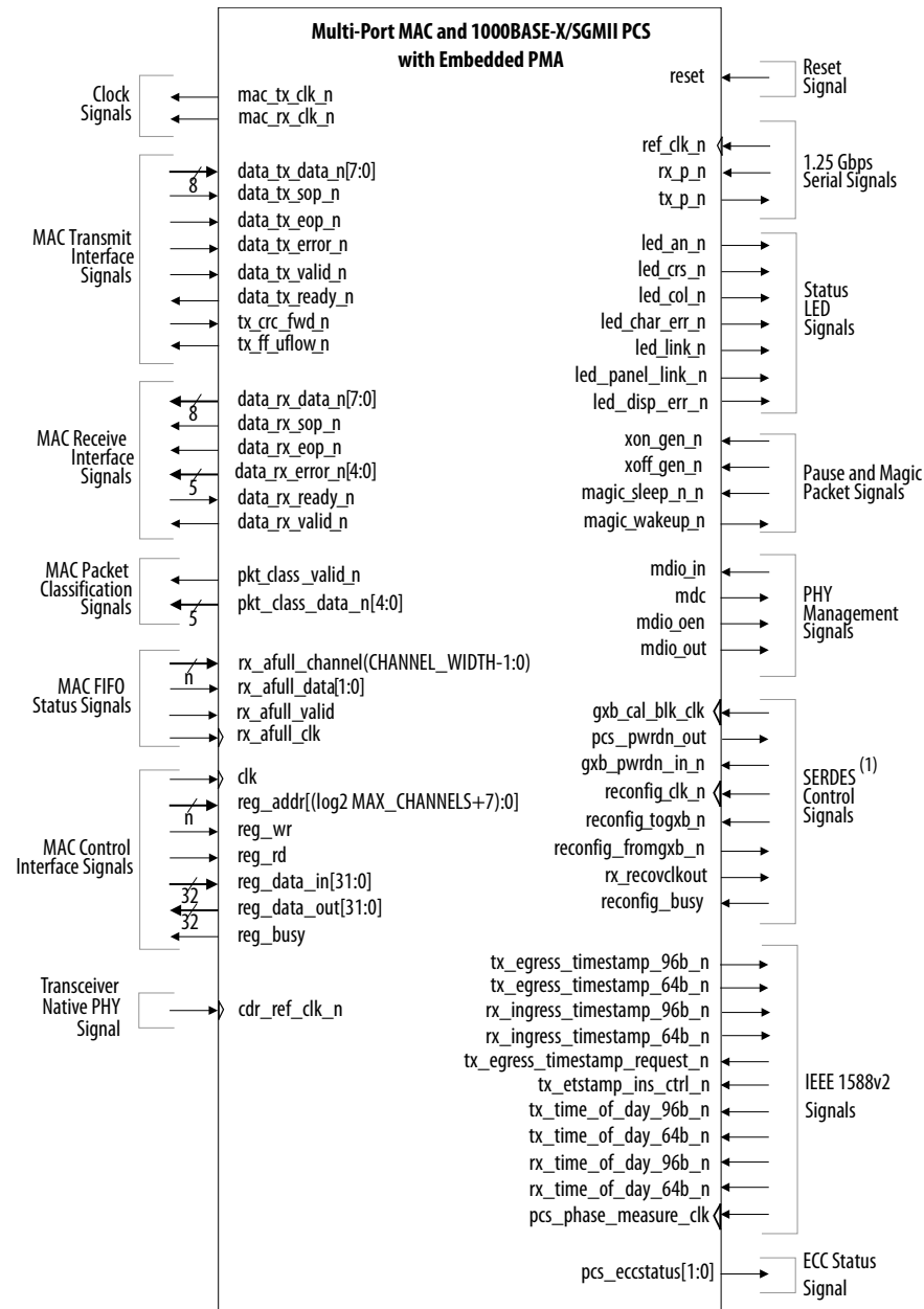
Figure 55. 10/100/1000 Multiport Ethernet MAC Function without Internal FIFO Buffers, with IEEE 1588v2, 1000BASE-X/SGMII PCS and Embedded PMA Signals
