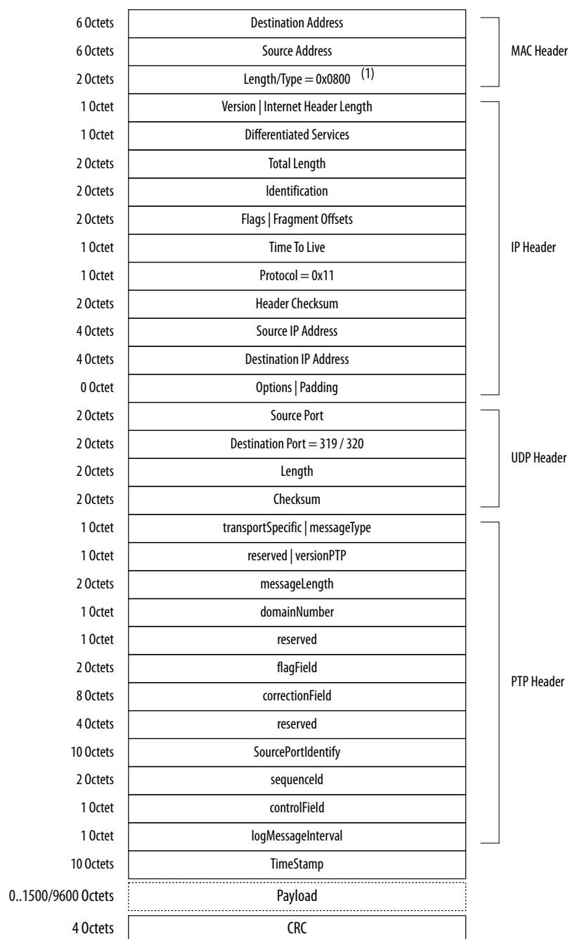
Figure 41. PTP Frame over UDP/IPv4
