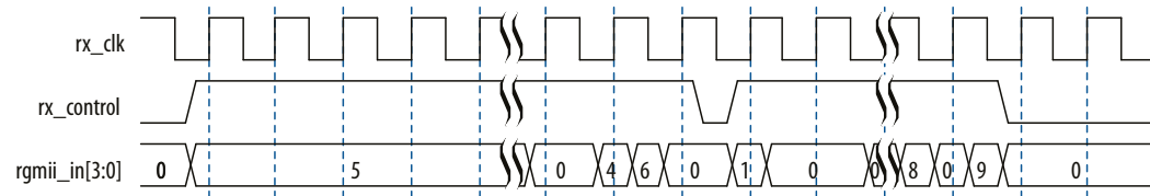
Figure 71. RGMII Receive with Error in Gigabit Mode
