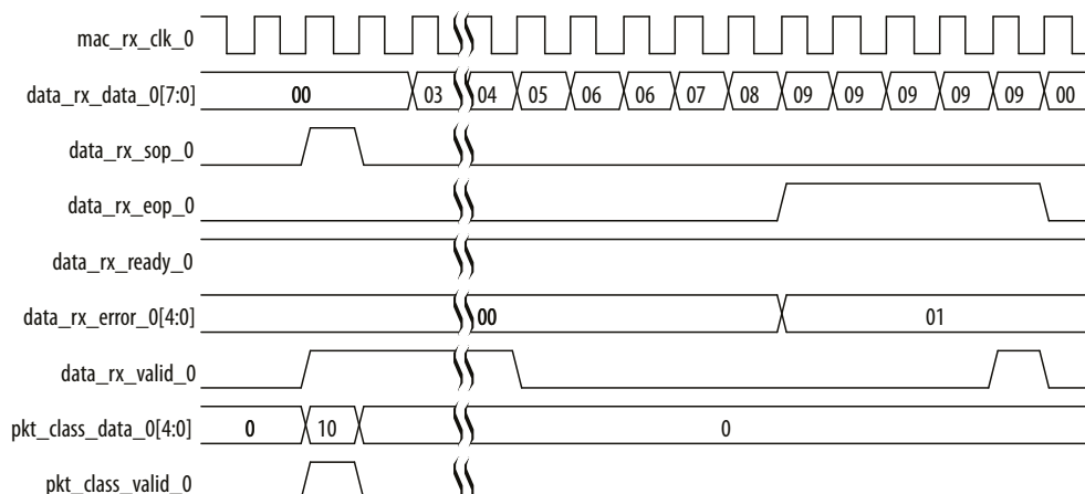
Figure 63. Invalid Length Error During Receive Operation—MAC Without Internal FIFO Buffers
