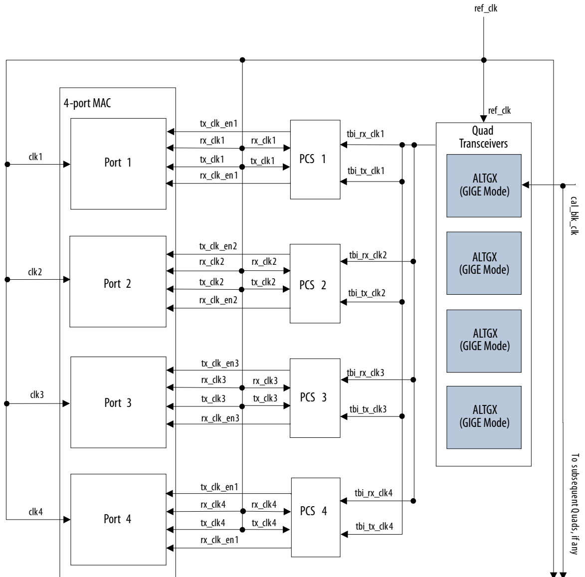
Figure 76. Clock Distribution in MAC and SGMII PCS with GXB Configuration—Optimal Case
