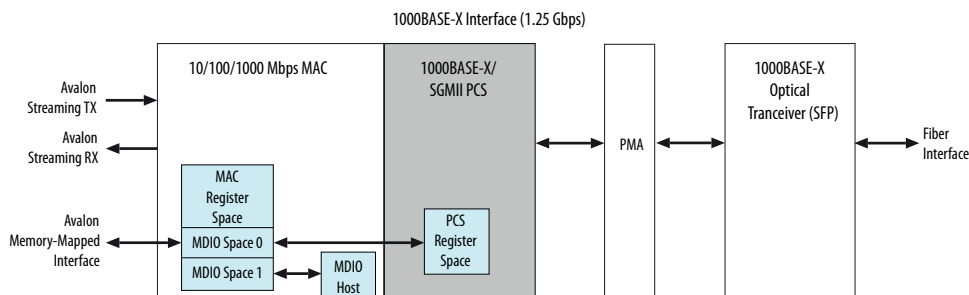
Figure 46. Triple-Speed Ethernet System with 1000BASE-X Interface with Register Initialization Recommendation
