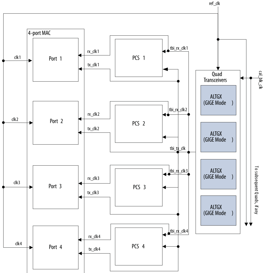
Figure 77. Clock Distribution in MAC and 1000BASE-X PCS with GXB Configuration—Optimal Case
