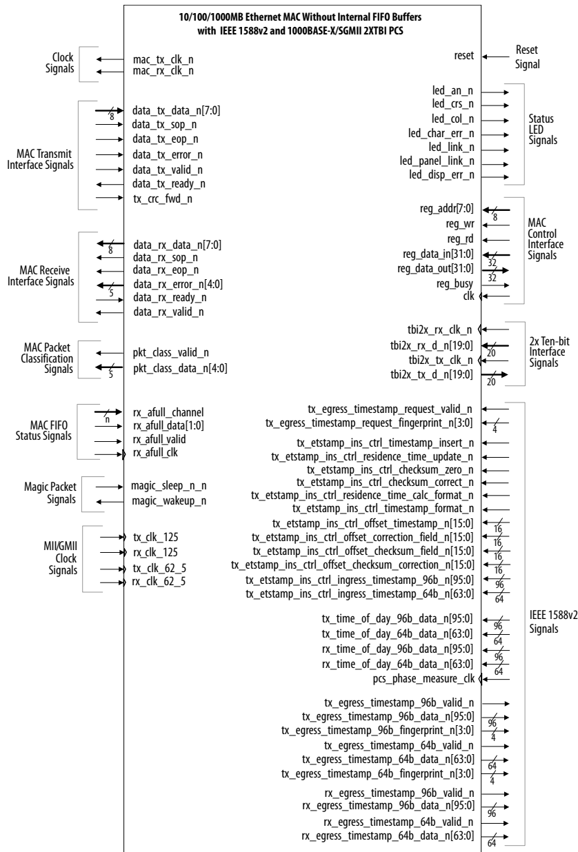
Figure 52. 10/100/1000 Ethernet MAC Function Without Internal FIFO Buffers with IEEE 1588v2 and 1000BASE-X/SGMII 2XTBI PCS Signals
