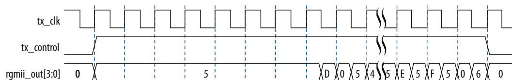
Figure 67. RGMII Transmit in Gigabit Mode
