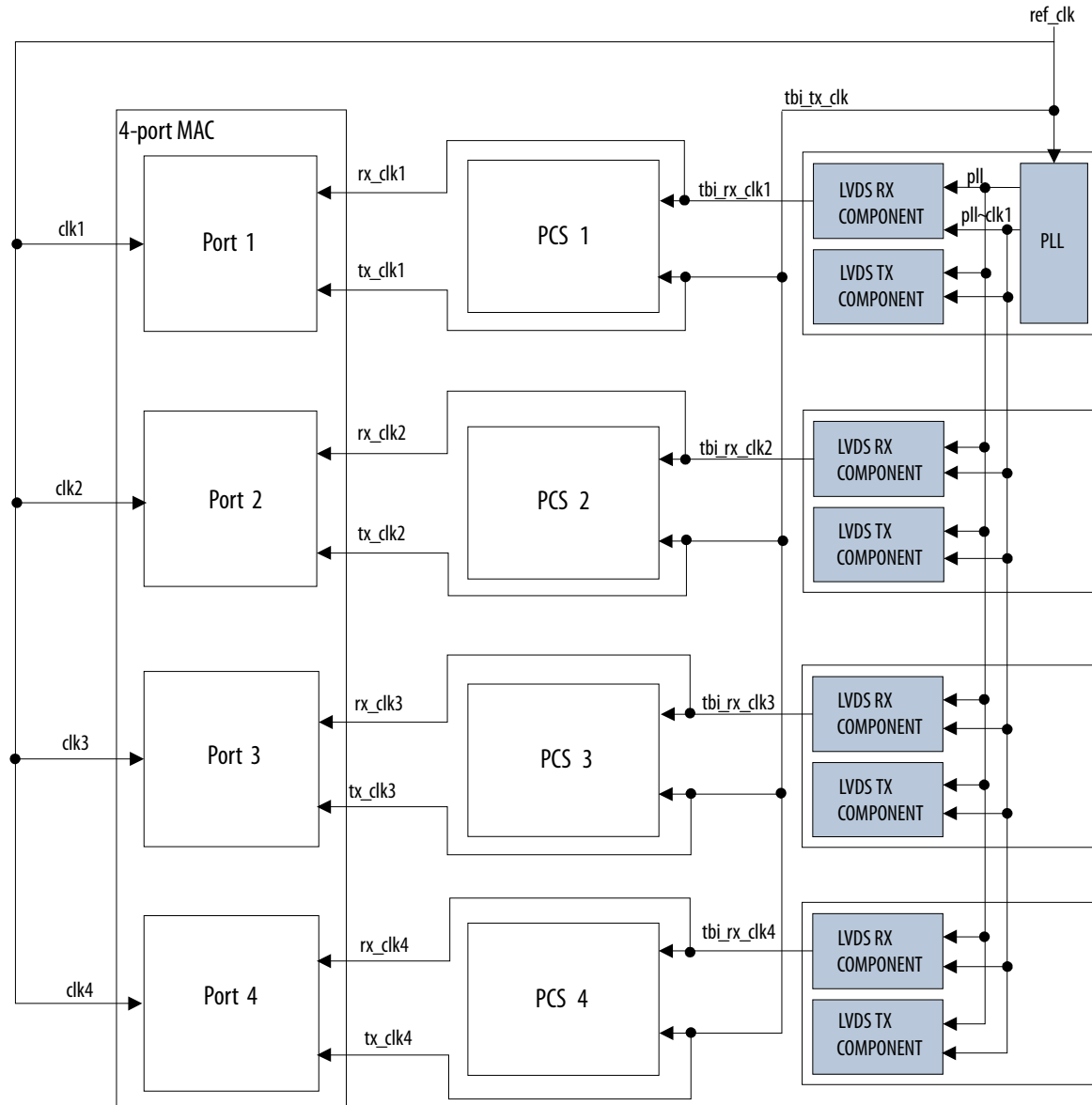
Figure 79. Clock Distribution in MAC and 1000BASE-X PCS with LVDS Configuration—Optimal Case
