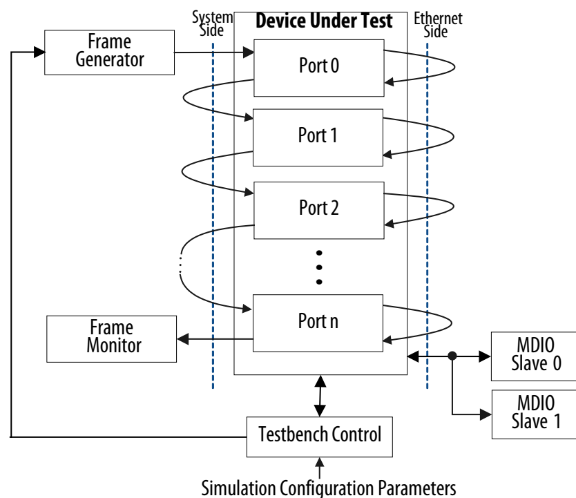
Figure 82. Triple-Speed Ethernet Testbench Architecture
