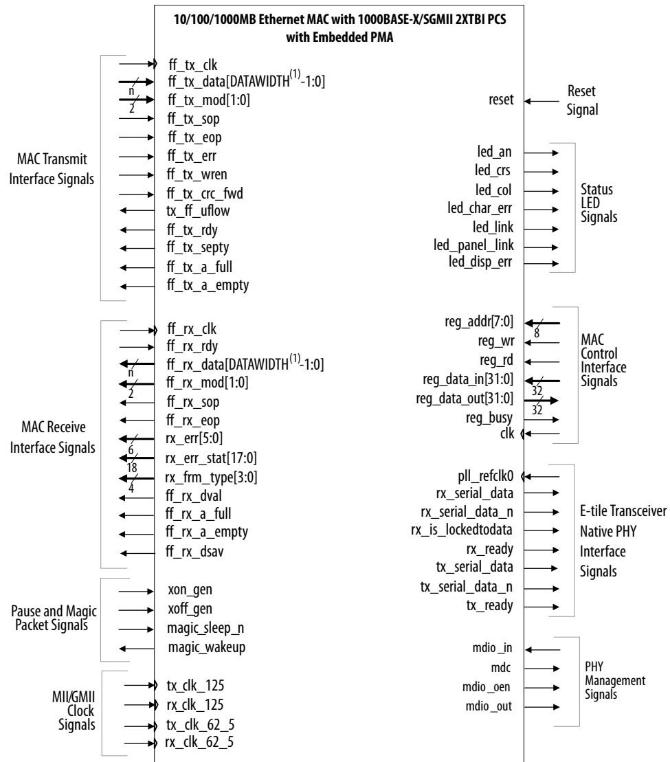
Figure 50. 10/100/1000 Ethernet MAC Function with Internal FIFO Buffers, and 1000BASE-X/SGMII 2XTBI PCS Signals With Embedded PMA Signals
