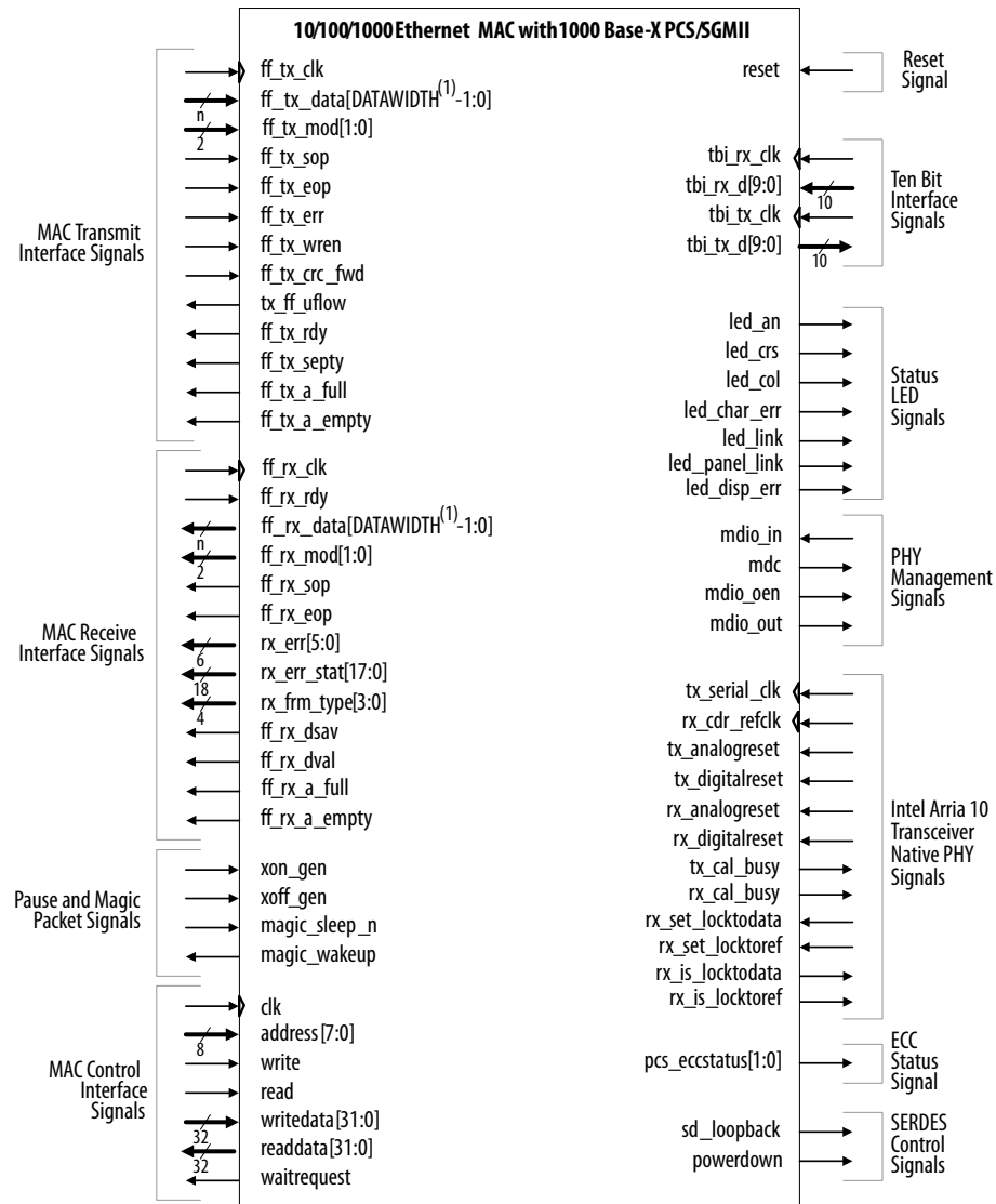
Figure 49. 10/100/1000 Ethernet MAC Function with Internal FIFO Buffers, with 1000BASE-X/SGMII PCS Signals
