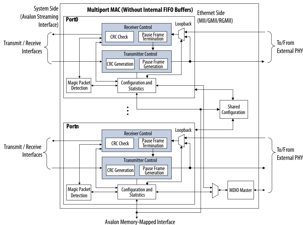
Figure 13. Multiport MAC Without Internal FIFO Buffers
