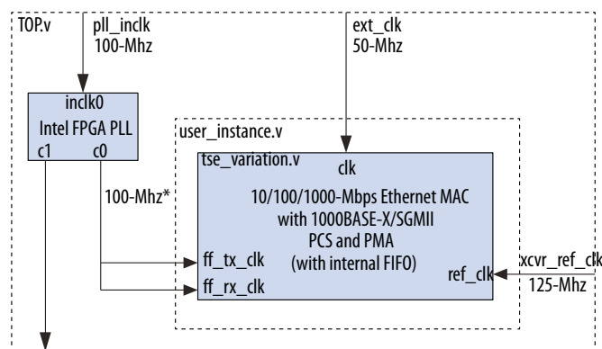
Figure 81. Triple-Speed Ethernet Timing Constraint Example
