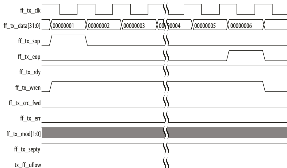
Figure 64. Transmit Operation—MAC With Internal FIFO Buffers
