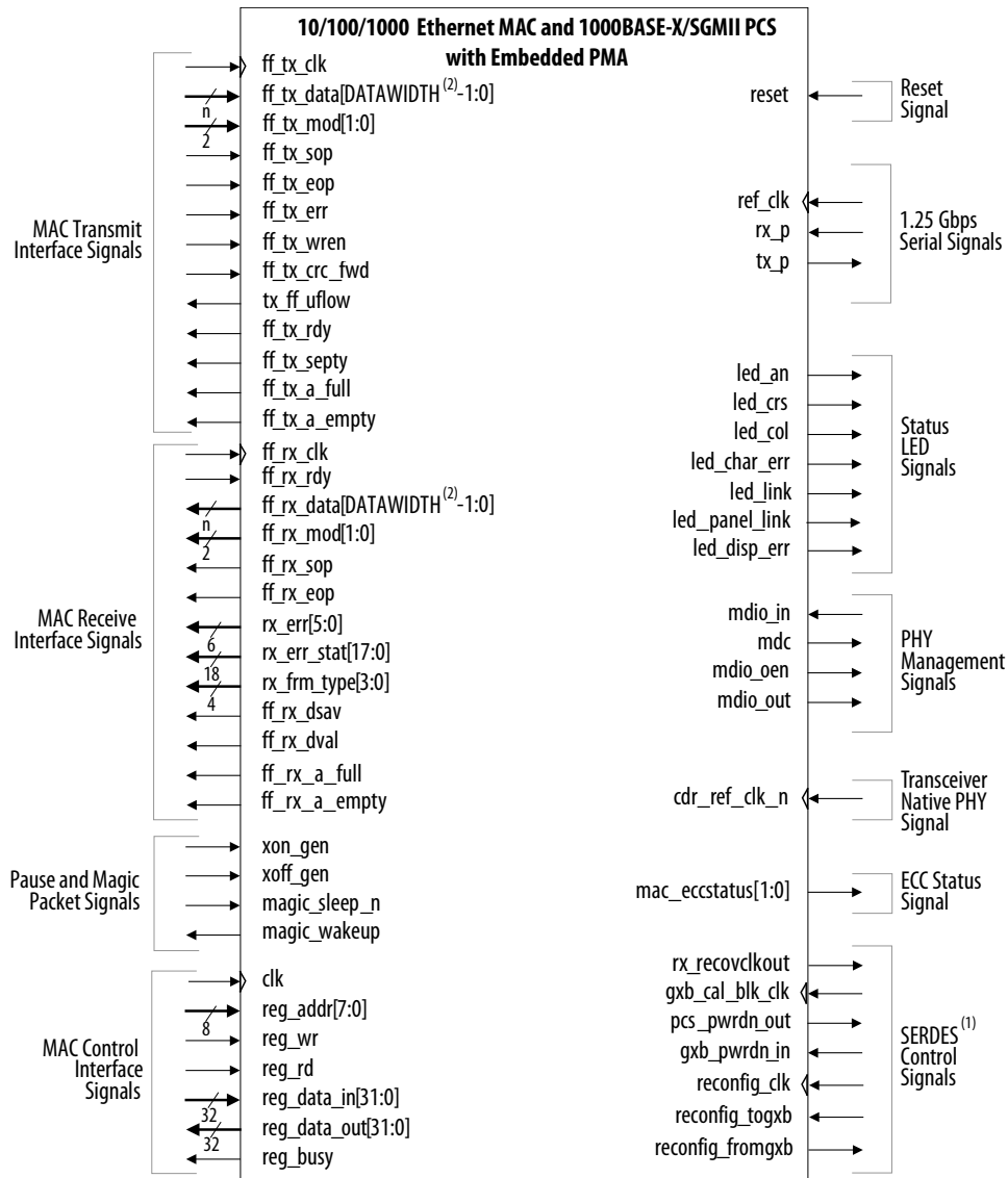
Figure 54. 10/100/1000 Ethernet MAC Function with Internal FIFO Buffers, and 1000BASE-X/SGMII PCS With Embedded PMA Signals
