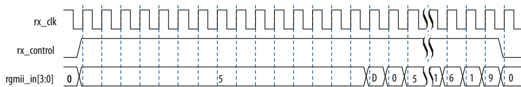
Figure 70. RGMII Receive in 1000 Mbps
