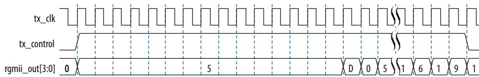
Figure 67. RGMII Transmit in Gigabit Mode
