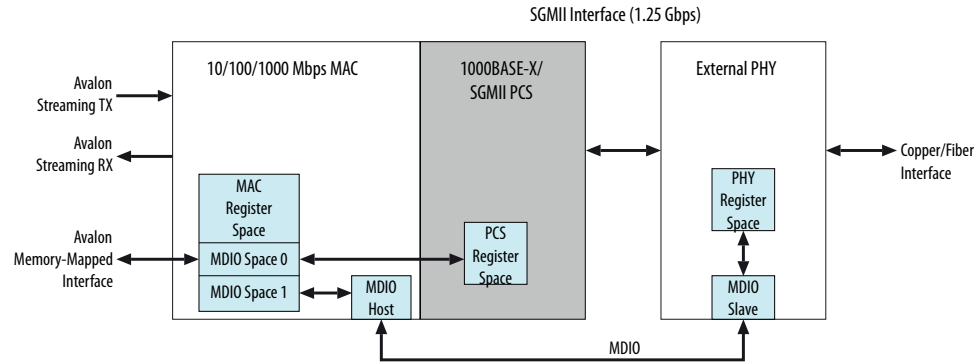
Figure 45. Triple-Speed Ethernet System with SGMII with Register Initialization Recommendation
