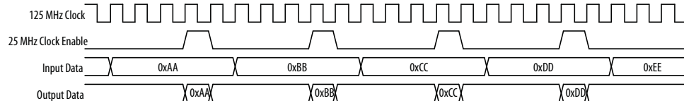
Figure 57. Clock Enabler Signal Behavior
