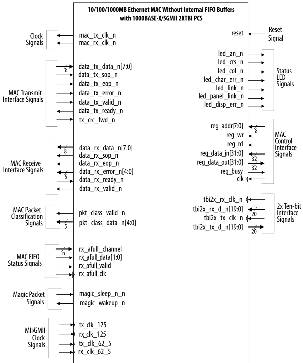
Figure 51. 10/100/1000 Ethernet MAC Function Without Internal FIFO Buffers with 1000BASE-X/SGMII 2XTBI PCS Signals
