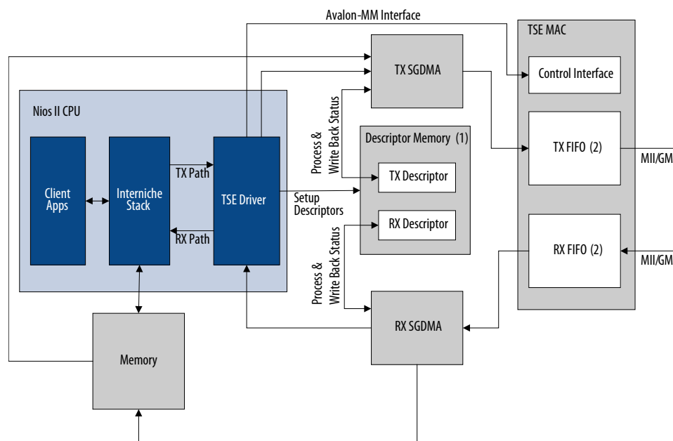
Figure 83. Triple-Speed Ethernet Software Driver Architecture
