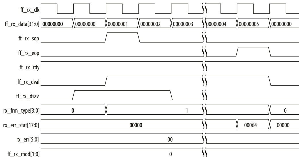
Figure 60. Receive Operation—MAC With Internal FIFO Buffers
