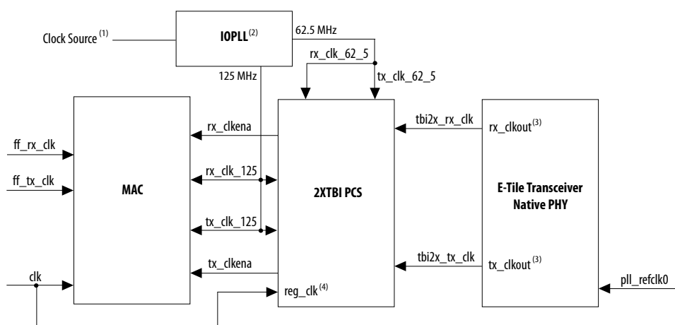
Figure 80. Clock Connectivity in MAC with 2XTBI PCS and Embedded PMA
