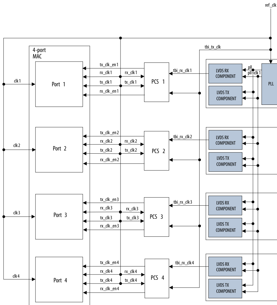
Figure 78. Clock Distribution in MAC and SGMII PCS with LVDS Configuration—Optimal Case
