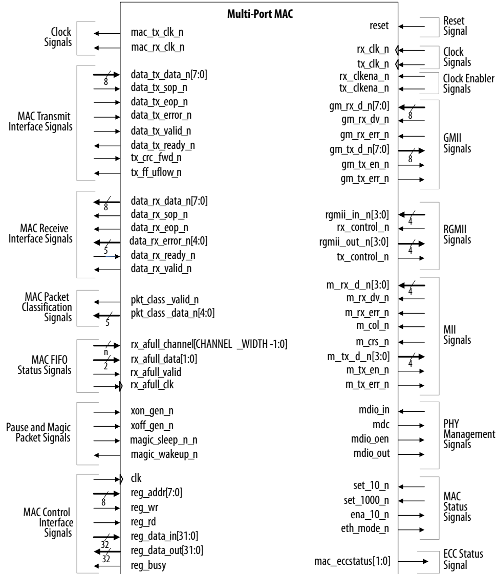
Figure 48. 10/100/1000 Multiport Ethernet MAC Function without Internal FIFO Buffers Signals
