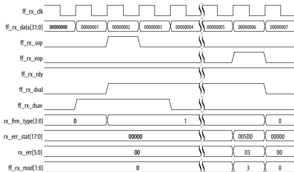
Figure 62. Invalid Length Error During Receive Operation—MAC With Internal FIFO Buffer
