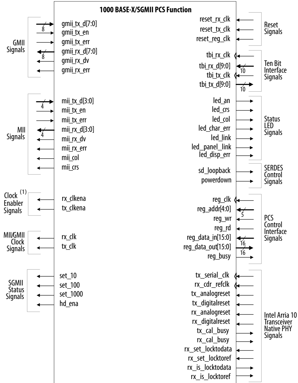
Figure 56. 1000BASE-X/SGMII PCS Function Signals
