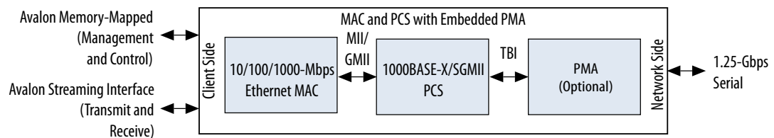
Figure 3. 10/100/1000 Mbps Ethernet MAC and 1000BASE-X/SGMII PCS with Optional PMA
