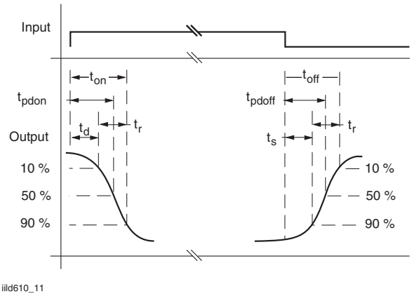
Fig. 11 - Saturated Switching Time Test Waveform
