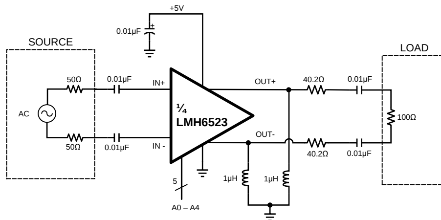
Figure 44. LMH6523 Basic Connections Schematic
