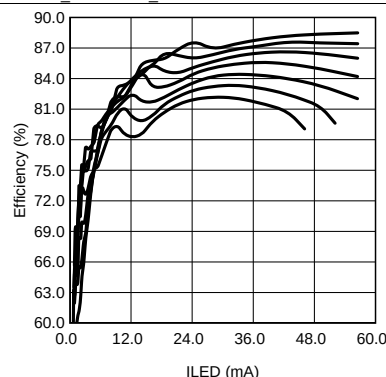
L = 10\text{ }\mu\text{H} V_{IN} = 3.6\text{ V} f_{SW} = 1\text{ MHz} Top To Bottom: 2×4, 2×5, 2×6, 2×7, 2×8, 2×9, 2×10 (LEDs)
