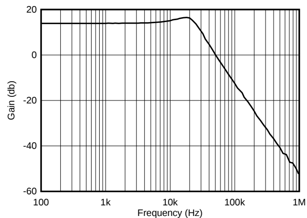
Figure 45. Gain (dB) vs Frequency (Hz)
