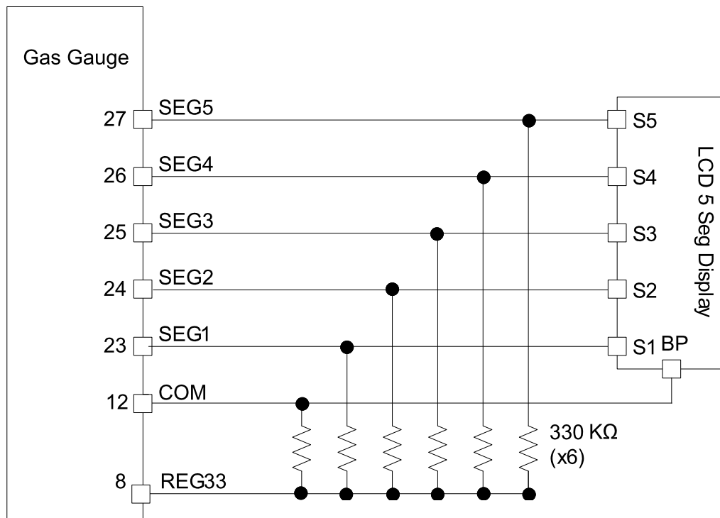
Figure 4. Typical LCD Implementation
