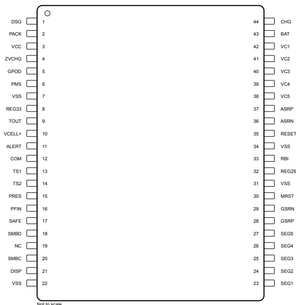
Pin Functions
