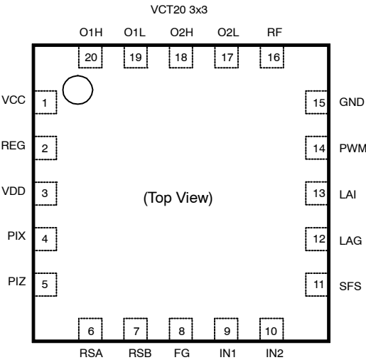
Figure 4. LV88551R, LV88552R, LV88553R, LV88554R Pin Assignment
