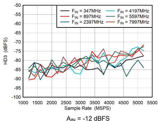
Figure 6-55. Dual Channel Mode: HD3 vs Sample Rate
