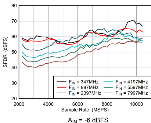
Figure 6-33. DES Mode: SFDR vs Sample Rate
