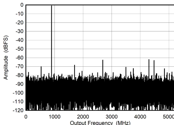
Figure 6-6. DES Mode: Single Tone FFT at 897 MHz
