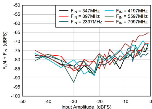
Figure 6-67. DES Mode: F_S/4 + F_{\text{IN}} vs Input Amplitude
