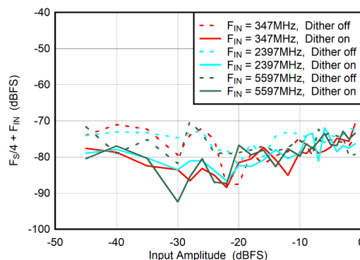
Figure 6-68. DES Mode: F_S/4 + F_{\text{IN}} vs Input Amplitude and Dither
