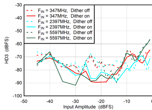
Figure 6-64. DES Mode: HD3 vs Input Amplitude and Dither
