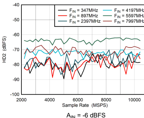
Figure 6-36. DES Mode: HD2 vs Sample Rate
