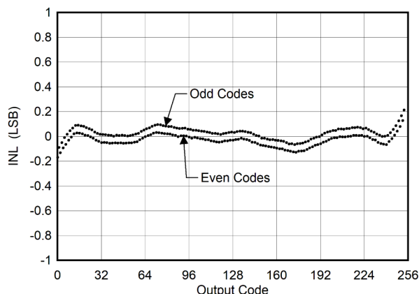
Figure 6-4. INL vs ADC Code
