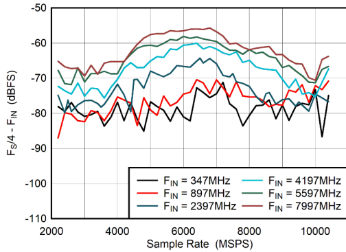
Figure 6-43. DES Mode: F_S/4 - F_{\text{IN}} vs Sample Rate
