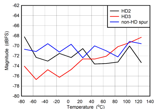
Figure 6-90. Dual Channel Mode: HD2, HD3 and Worst Spur vs Temperature
