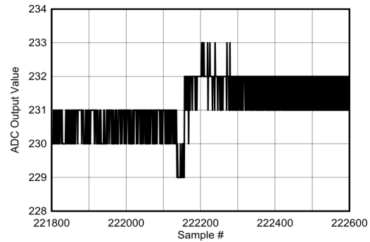
Figure 6-122. Background Calibration Core Transition (DC Signal Zoomed)
