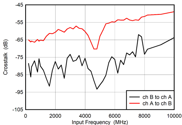
Figure 6-2. Crosstalk vs Input Frequency
