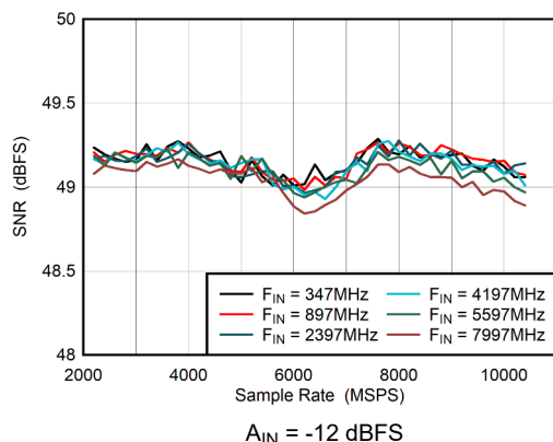
Figure 6-31. DES Mode: SNR vs Sample Rate
