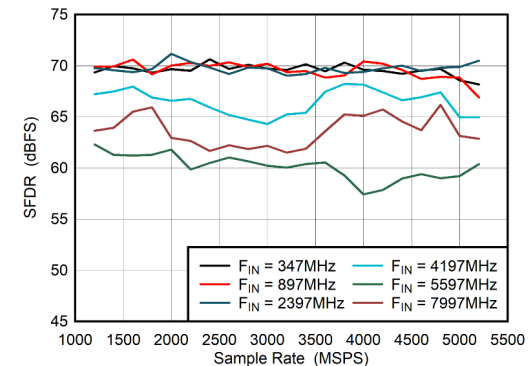
Figure 6-48. Dual Channel Mode: SFDR vs Sample Rate
