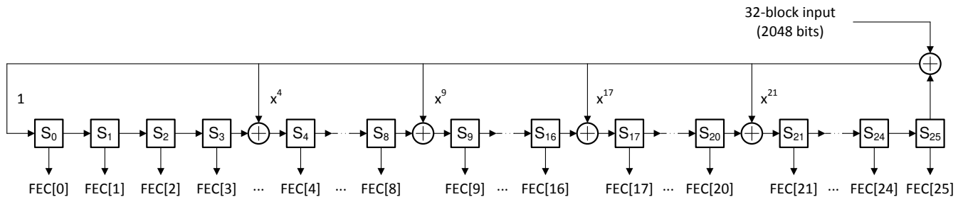
Figure 7-11. FEC Parity Bit Generator
