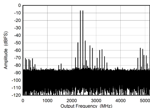
Figure 6-16. DES Mode: Two Tone FFT at 7997 MHz
