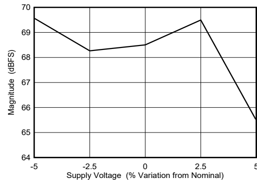
Figure 6-96. Dual Channel Mode: SFDR vs Supply Voltage
