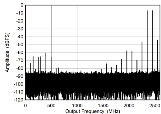
Figure 6-28. Dual Channel Mode: Two Tone FFT at 7997 MHz
