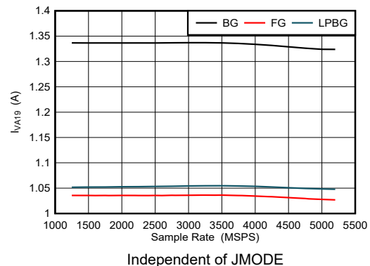
Figure 6-114. Dual Channel Mode: I_{VA19} vs Sample Rate
