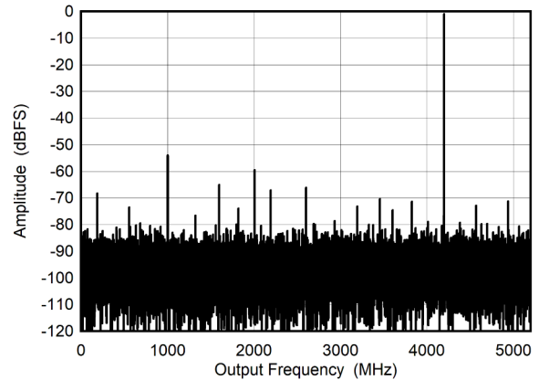
Figure 6-8. DES Mode: Single Tone FFT at 4197 MHz
