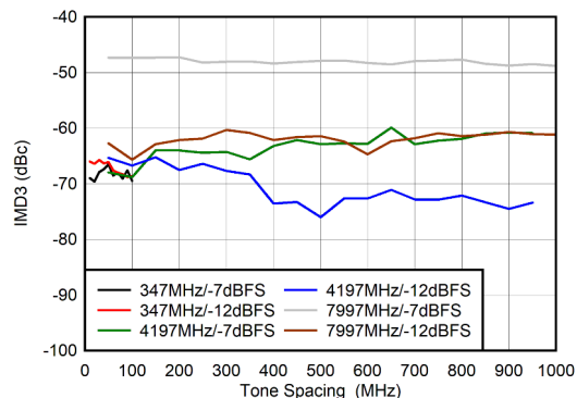
Figure 6-102. DES Mode: IMD3 vs Tone Spacing
