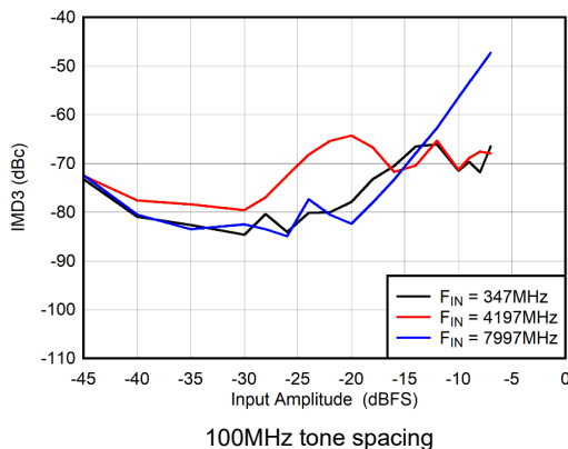
100MHz tone spacing Figure 6-101. DES Mode: IMD3 vs Input Amplitude
