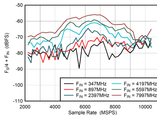
Figure 6-42. DES Mode: F_s/4 + F_{\text{IN}} vs Sample Rate
