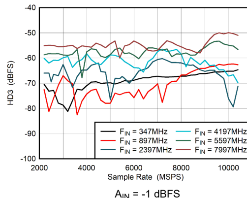
Figure 6-38. DES Mode: HD3 vs Sample Rate
