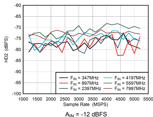
Figure 6-52. Dual Channel Mode: HD2 vs Sample Rate
