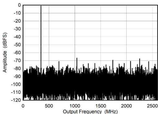
Figure 6-17. Dual Channel Mode: Single Tone FFT at 347 MHz
