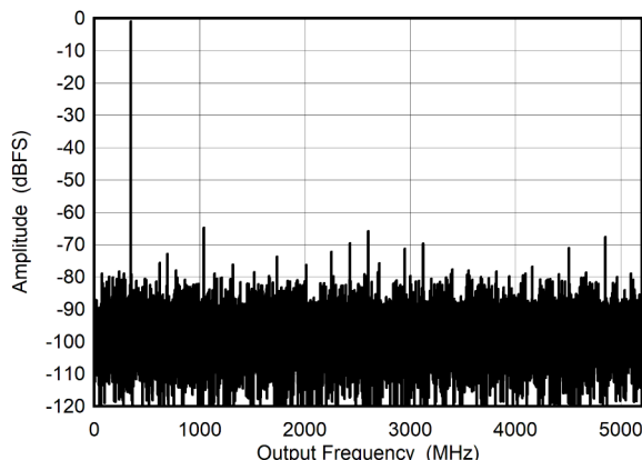
Figure 6-5. DES Mode: Single Tone FFT at 347 MHz
