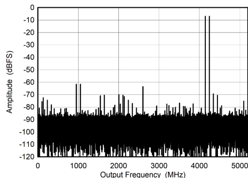
Figure 6-14. DES Mode: Two Tone FFT at 4197 MHz
