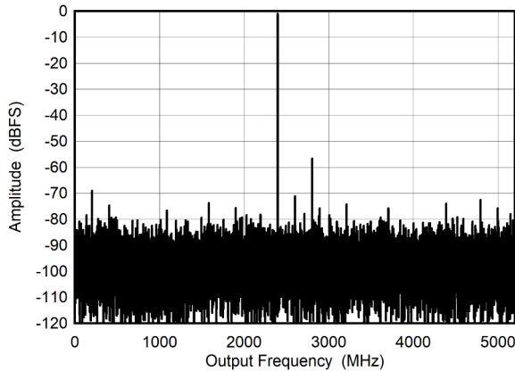
Figure 6-7. DES Mode: Single Tone FFT at 2397 MHz
