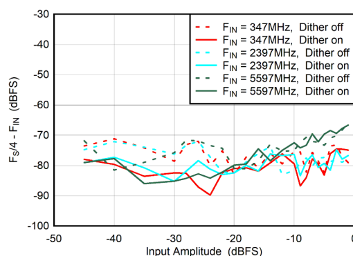
Figure 6-70. DES Mode: F_S/4 - F_{\text{IN}} vs Input Amplitude and Dither
