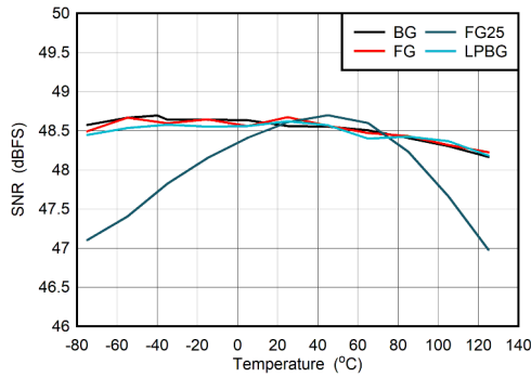
Figure 6-91. Dual Channel Mode: SNR vs Temperature and Calibration
