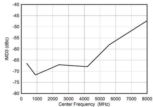
each tone -7\text{dBFS} , 100\text{MHz} tone spacing Figure 6-100. DES Mode: IMD3 vs Input Frequency
