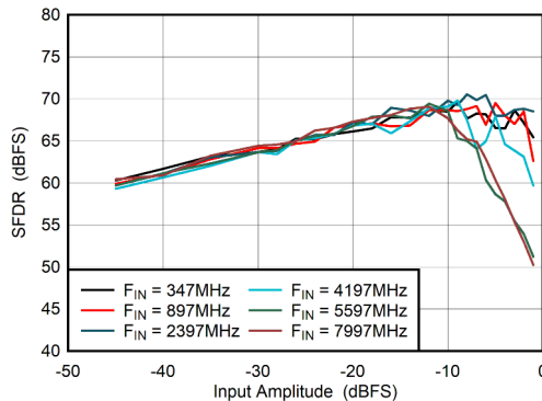
Figure 6-73. Dual Channel Mode: SFDR vs Input Amplitude
