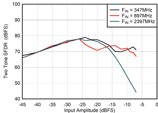
Figure 6-109. Dual Channel Mode: Two Tone SFDR vs Input Amplitude
