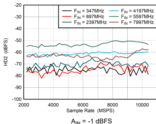
Figure 6-35. DES Mode: HD2 vs Sample Rate
