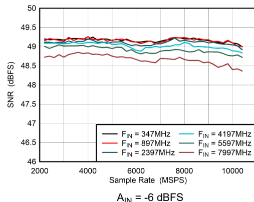
Figure 6-30. DES Mode: SNR vs Sample Rate
