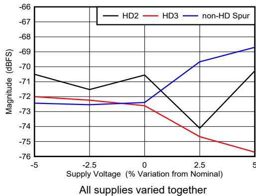
Figure 6-97. Dual Channel Mode: HD2, HD3 and Worst Spur vs Supply Voltage
