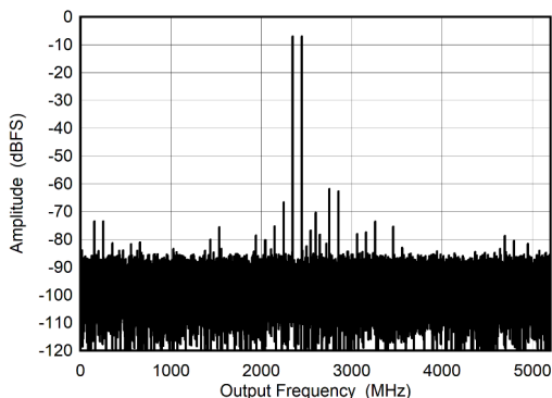
Figure 6-13. DES Mode: Two Tone FFT at 2397 MHz
