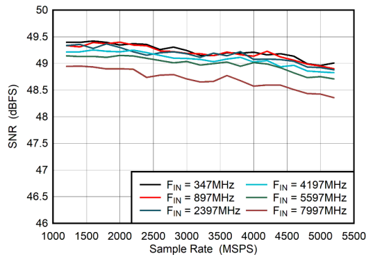
Figure 6-45. Dual Channel Mode: SNR vs Sample Rate
