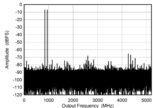
Figure 6-12. DES Mode: Two Tone FFT at 897 MHz
