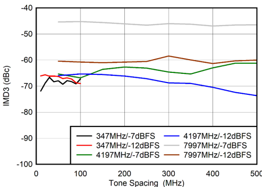
Figure 6-107. Dual Channel Mode: IMD3 vs Tone Spacing
