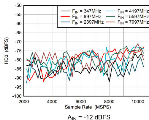
Figure 6-40. DES Mode: HD3 vs Sample Rate
