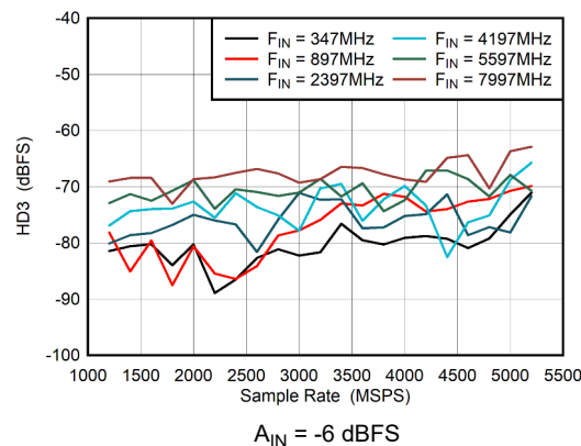
Figure 6-54. Dual Channel Mode: HD3 vs Sample Rate
