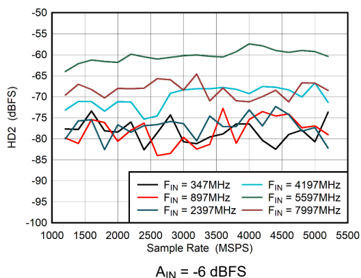
Figure 6-51. Dual Channel Mode: HD2 vs Sample Rate
