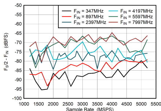
Figure 6-56. Dual Channel Mode: F_{\text{S}}/2 - F_{\text{IN}} vs Sample Rate
