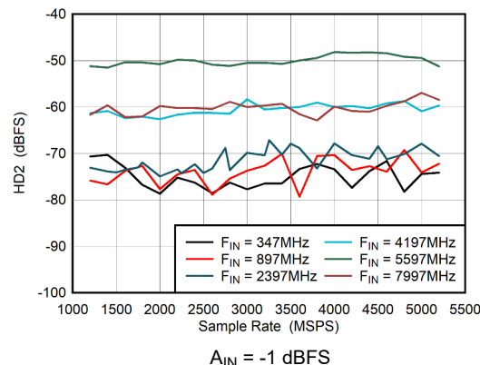
Figure 6-50. Dual Channel Mode: HD2 vs Sample Rate
