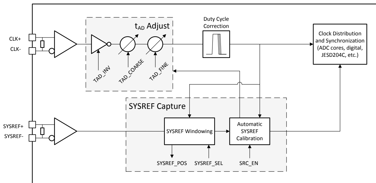
Figure 7-2. Clocking Subsystem
