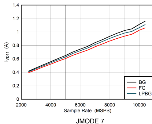
Figure 6-112. DES Mode: I_{VD11} vs Sample Rate
