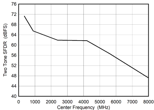
Figure 6-103. DES Mode: Two Tone SFDR vs Input Frequency
