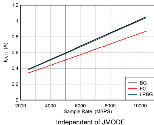
Figure 6-111. DES Mode: I_{VA11} vs Sample Rate
