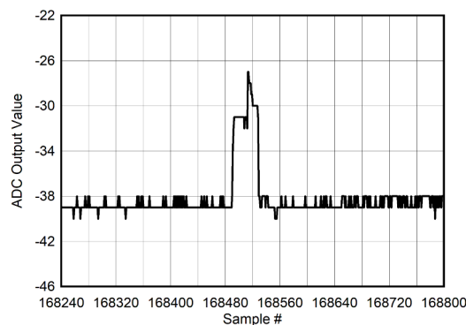
Figure 6-120. Background Calibration Core Transition (AC Signal Zoomed)
