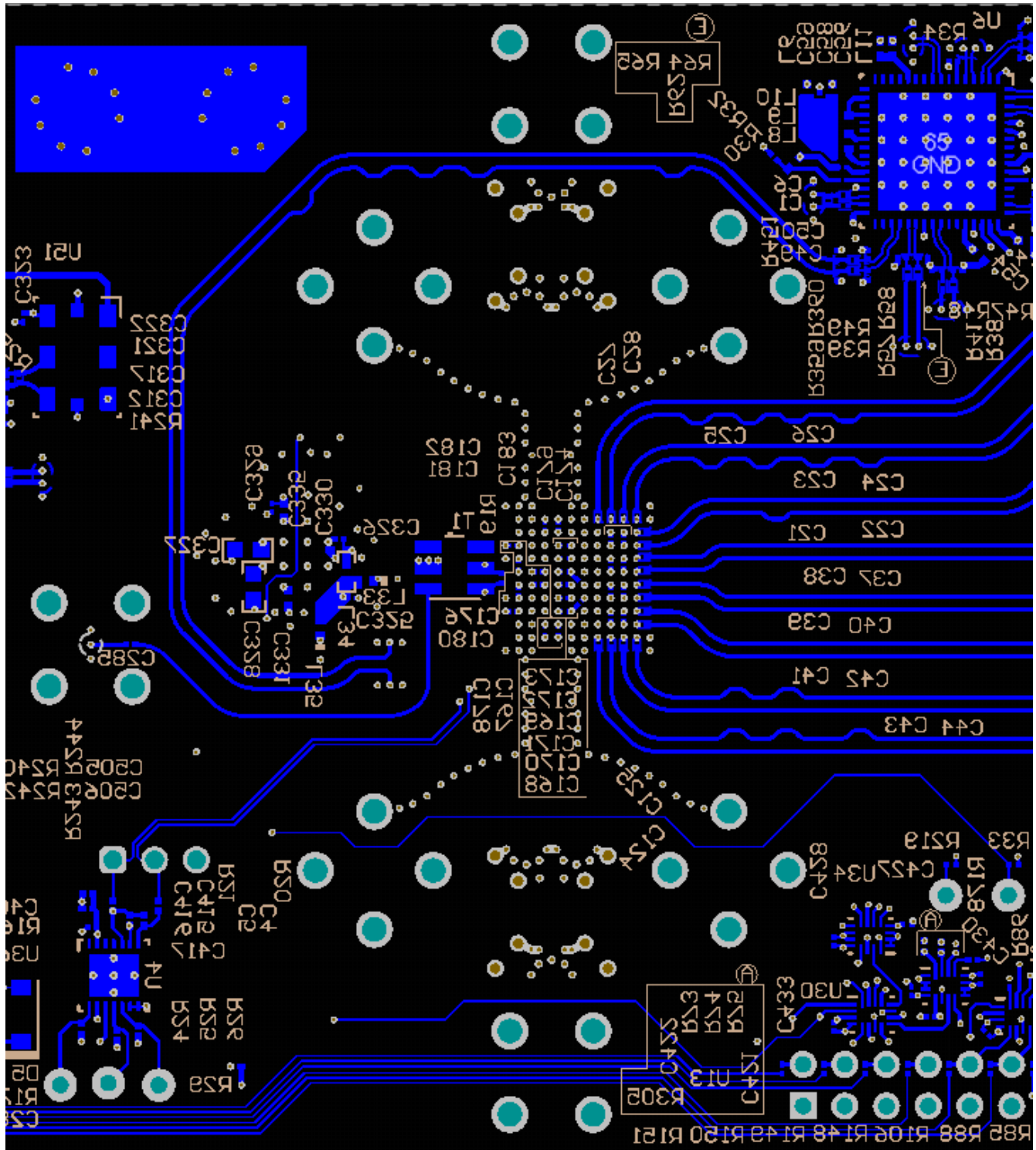
Figure 10-3. Bottom Layer Routing: Additional CLK Routing, DA4-7, DB4-7
