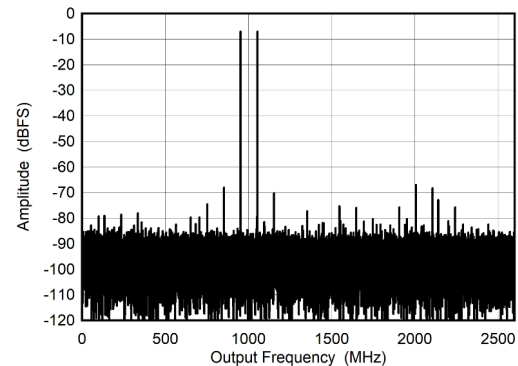
Figure 6-26. Dual Channel Mode: Two Tone FFT at 4197 MHz
