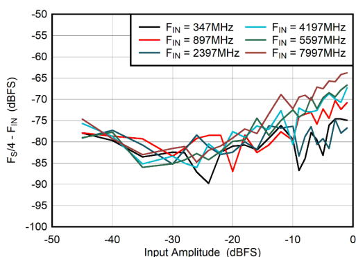
Figure 6-69. DES Mode: F_S/4 - F_{\text{IN}} vs Input Amplitude
