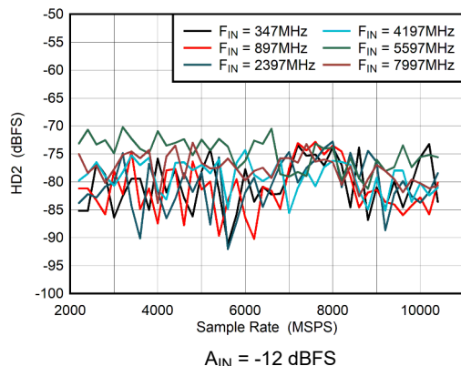
Figure 6-37. DES Mode: HD2 vs Sample Rate
