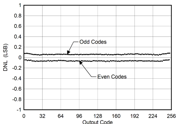
Figure 6-3. DNL vs ADC Code
