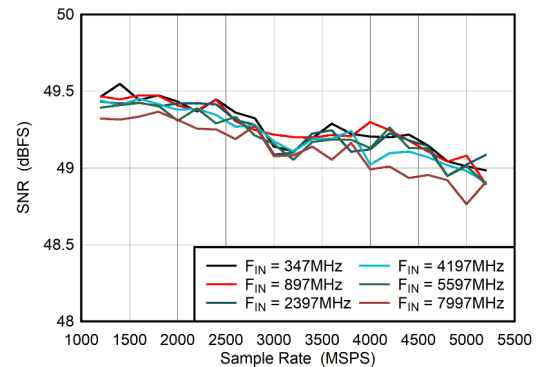
Figure 6-46. Dual Channel Mode: SNR vs Sample Rate
