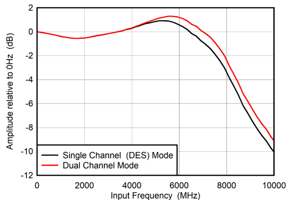
Figure 6-1. Input Amplitude vs Input Frequency
