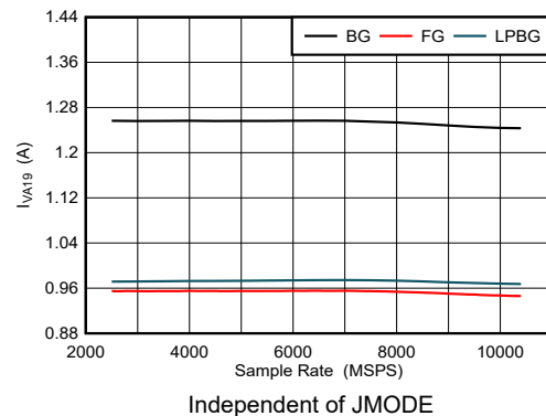
Figure 6-110. DES Mode: I_{VA19} vs Sample Rate
