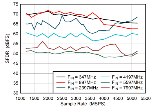
Figure 6-47. Dual Channel Mode: SFDR vs Sample Rate
