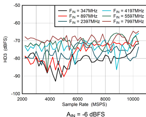
Figure 6-39. DES Mode: HD3 vs Sample Rate
