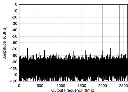
Figure 6-19. Dual Channel Mode: Single Tone FFT at 2397 MHz
