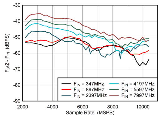
Figure 6-41. DES Mode: F_s/2 - F_{\text{IN}} vs Sample Rate
