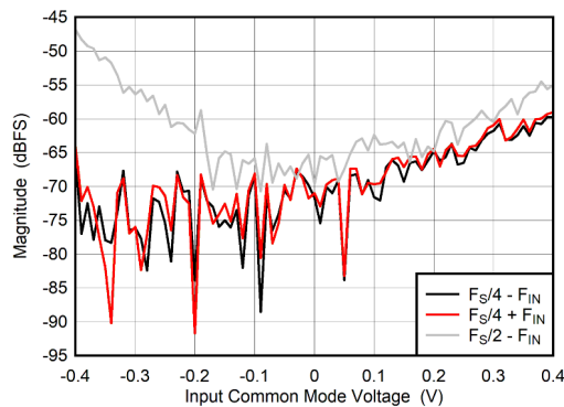
Figure 6-99. DES Mode: F_S/2 - F_{\text{IN}} , F_S/4 \pm F_{\text{IN}} vs Input Common Mode Voltage
