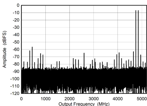
Figure 6-15. DES Mode: Two Tone FFT at 5597 MHz
