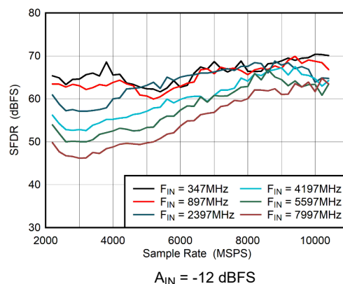
Figure 6-34. DES Mode: SFDR vs Sample Rate
