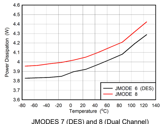
Figure 6-118. Power Dissipation vs Temperature
