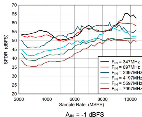
Figure 6-32. DES Mode: SFDR vs Sample Rate
