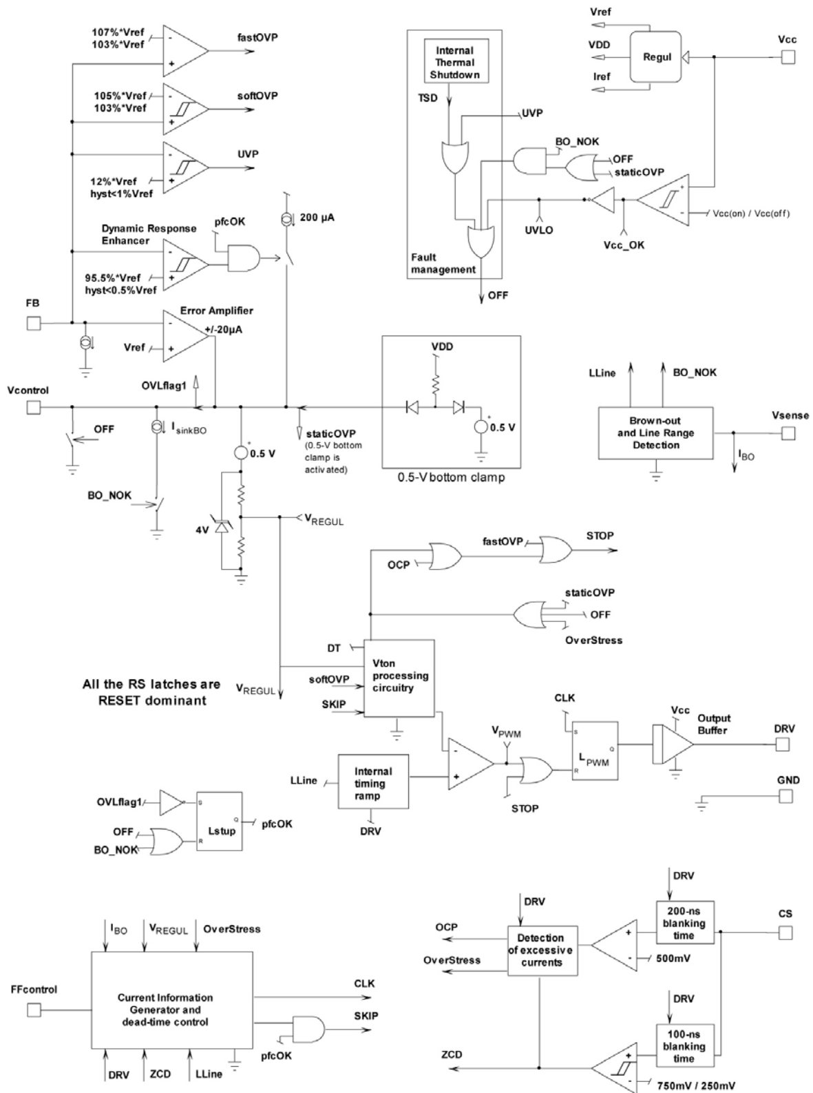
Figure 2. Block Diagram
