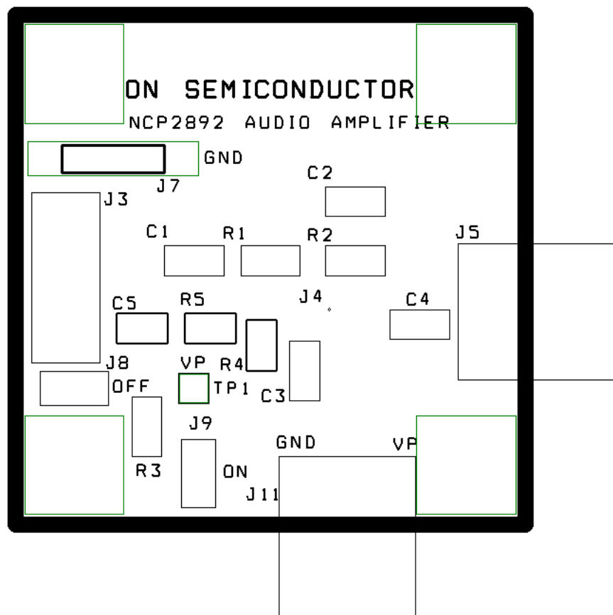
Figure 35. Demonstration Board for 9-Pin Flip-Chip CSP Device – PCB Layers
